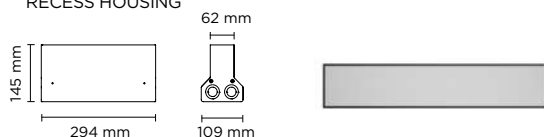
RECESS HOUSING
