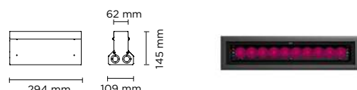
RECESS HOUSING
