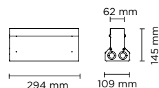
RECESS HOUSING
