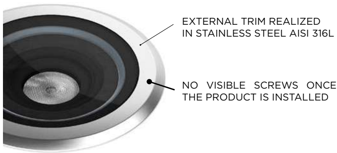
REDUCED WIDTH AT 20 MM FOR BETTER AESTHETIC IMPACT
