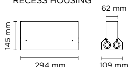
RECESS HOUSING
