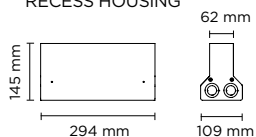
RECESS HOUSING
